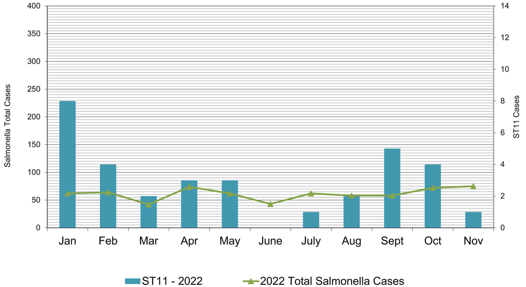
NZ Monthly Salmonella ST11vs Total Cases
